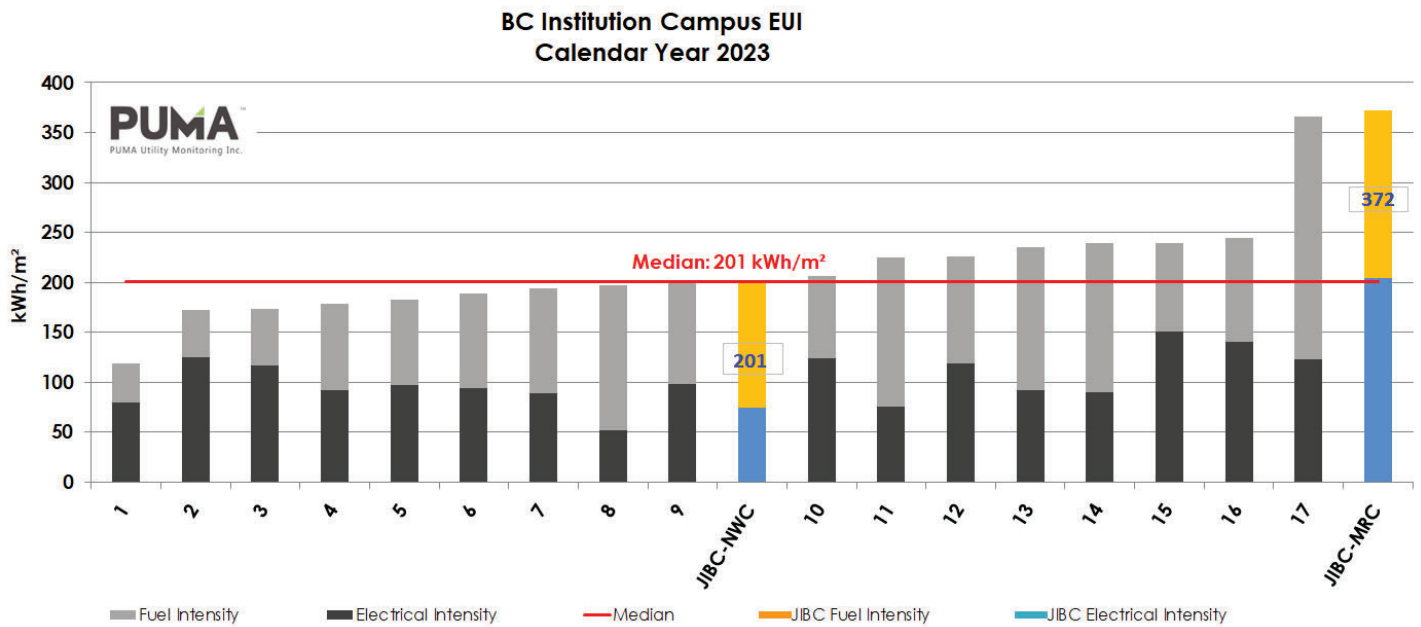
Figure 6: Benchmarking Comparison to Other Post-Secondary Institutions in BC
