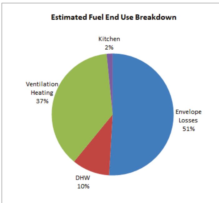
Figure 5: Gas End-Use Breakdown for New Westminster Campus (2018)
